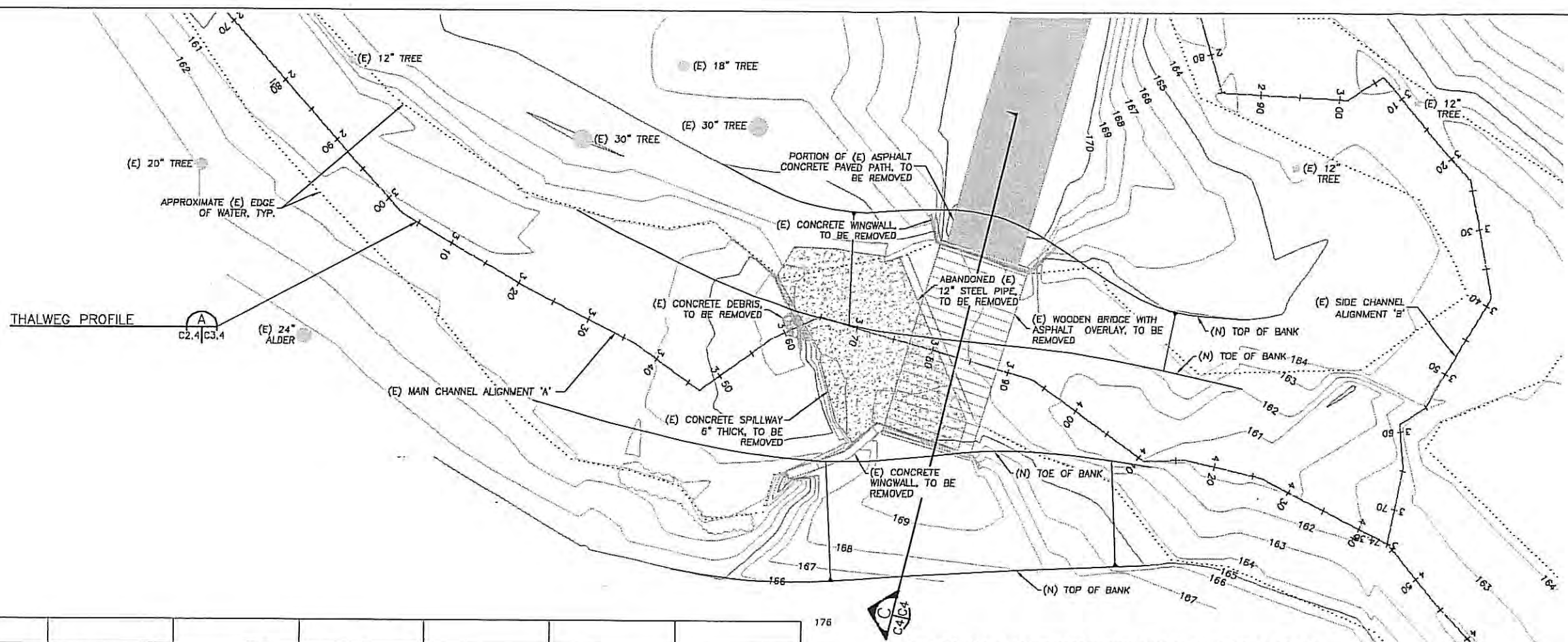
SITE PLAN - ALTERNATIVE #2 (BRIDGE REMOVAL) SCALE: 1"=8'
