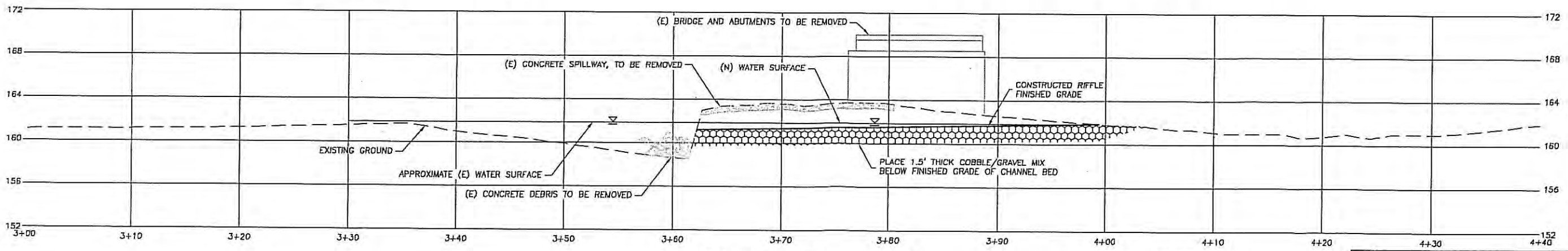
THALWEG PROFILE SCALE: 1"=5' H; 1"=5' V
