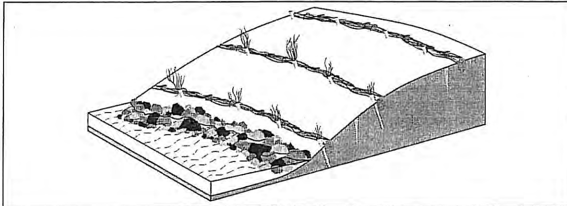
Figure 4-9. Live Fascine/Wattles
