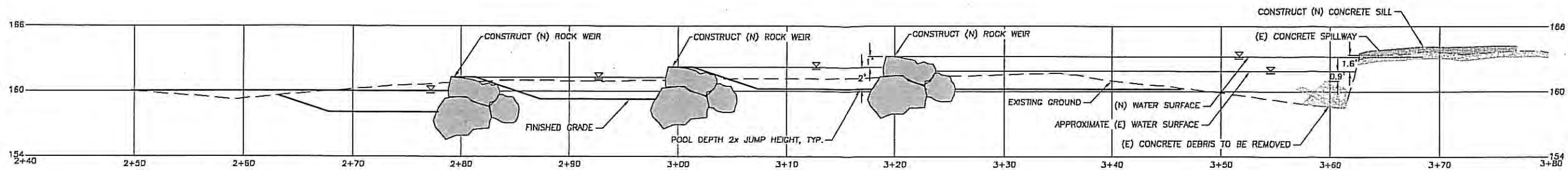
THALWEG PROFILE SCALE: 1"=5' H; 1"=5' V
