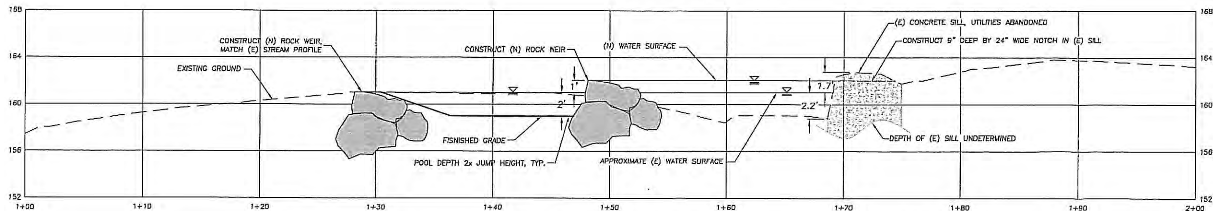
THALWEG PROFILE SCALE: 1"=4' H; 1"=4' V
