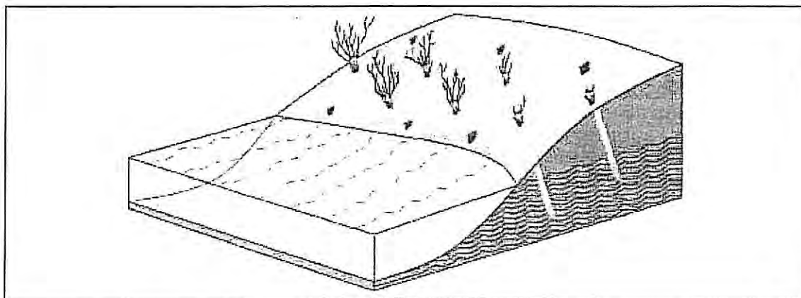
Figure 4-10. Live Stakes
