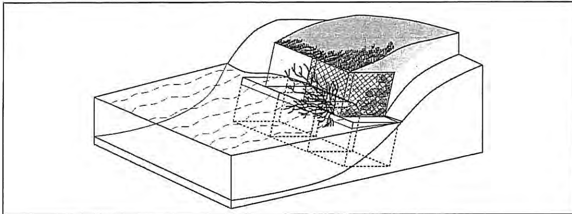
Figure 4-12. Vegetated Gabions
