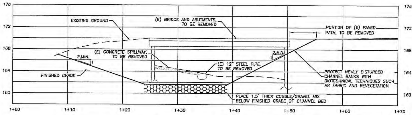
BRIDGE SECTION SCALE: 1"=5' H; 1"=5' V
